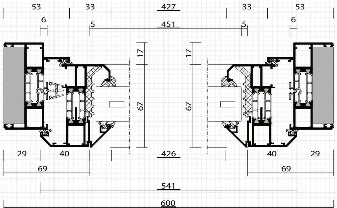
Top Cross Section
